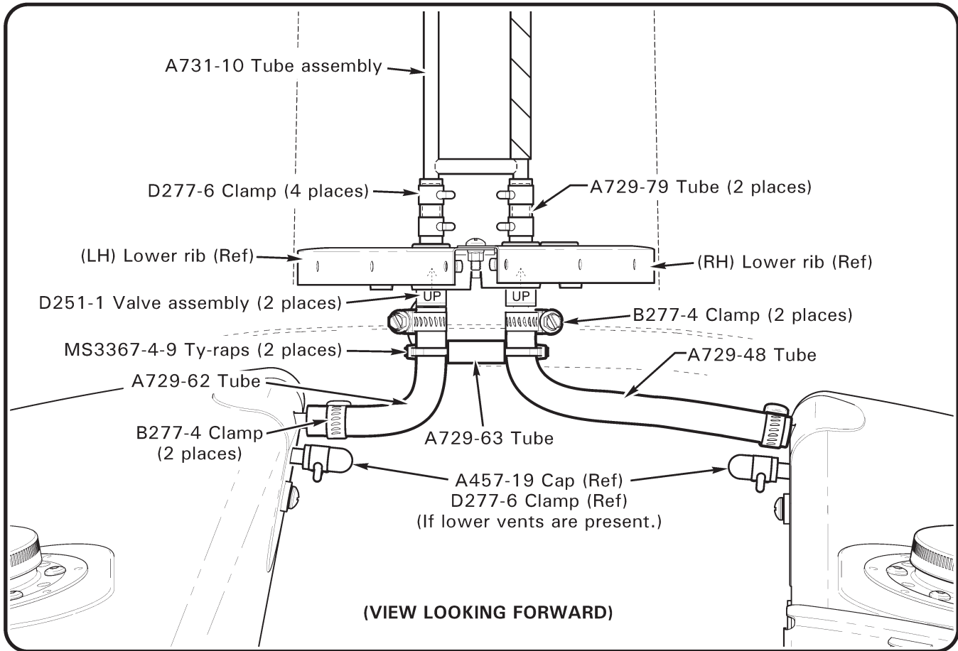
FIGURE 4 Upgraded fuel tank venting system
