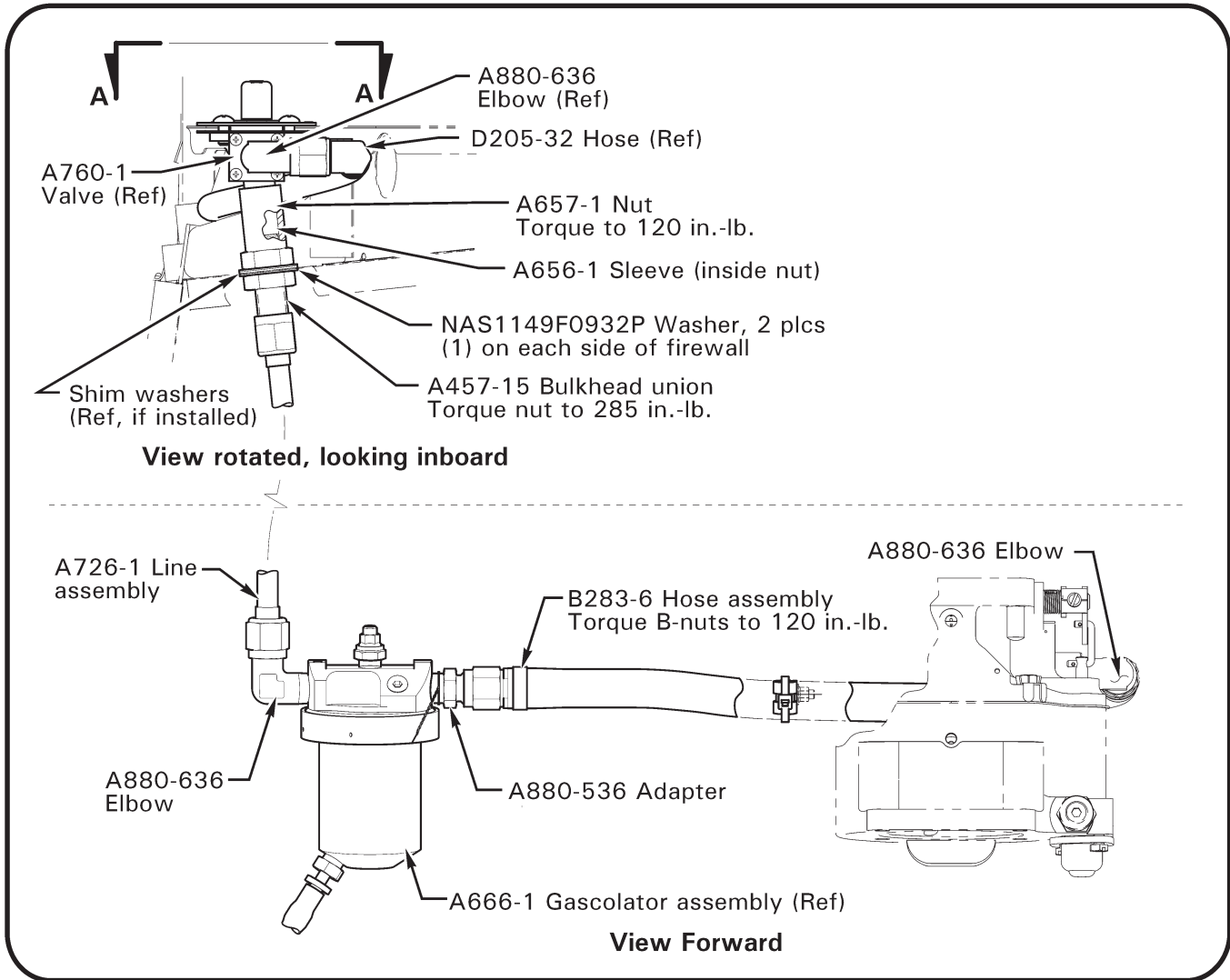
FIGURE 1 Installation of A880-series parts
