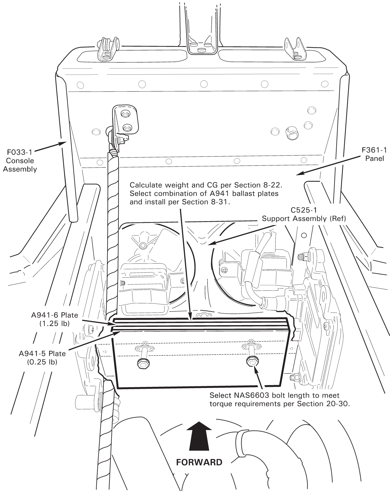
FIGURE 8-4 NOSE BALLAST
